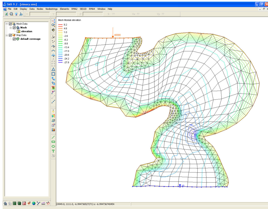
Figure 1. The mesh from stmary.sms.
