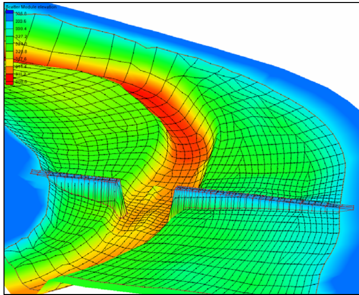
Figure 6 Mesh incorporating the east and west abutments.
