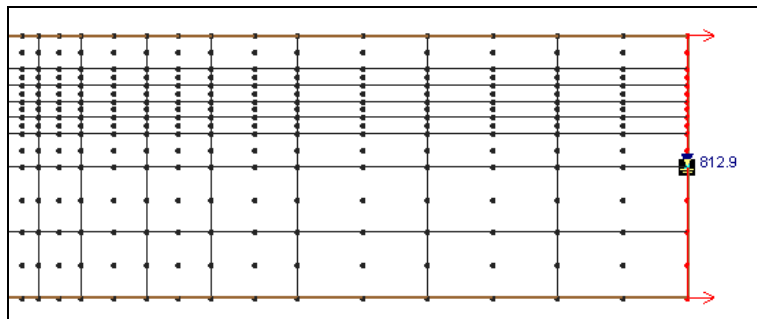
Figure 4 The outflow boundary condition.
